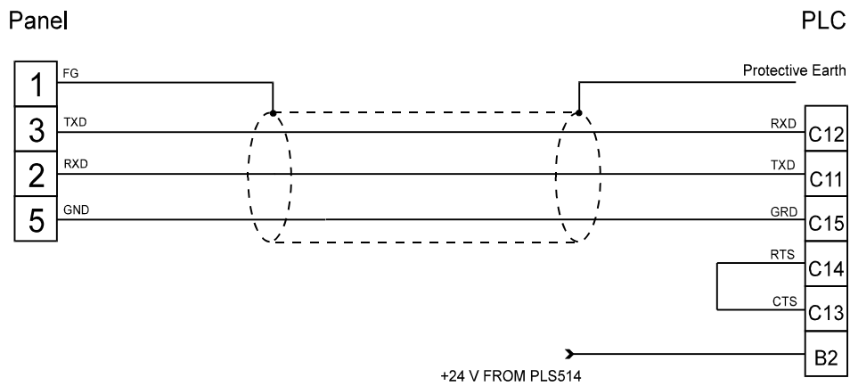
figure 1. Cable diagram
