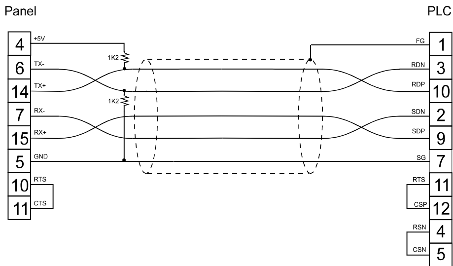
figure 1. Cable diagram
