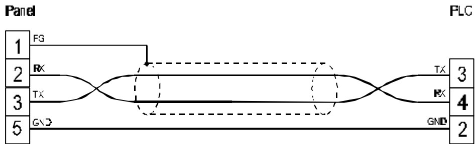
Figure 1. Cable diagram
