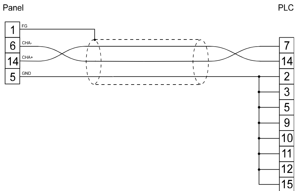
figure 1. Cable diagram
