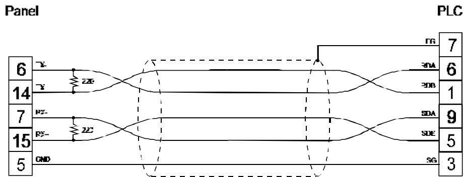
figure 1. Cable diagram
