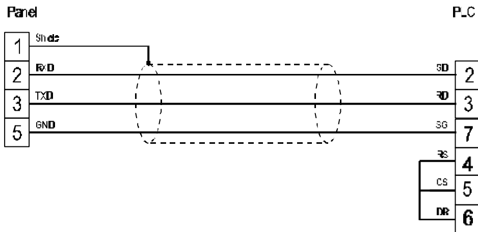
figure 1. Cable diagram
