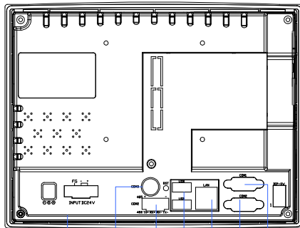
Connections
