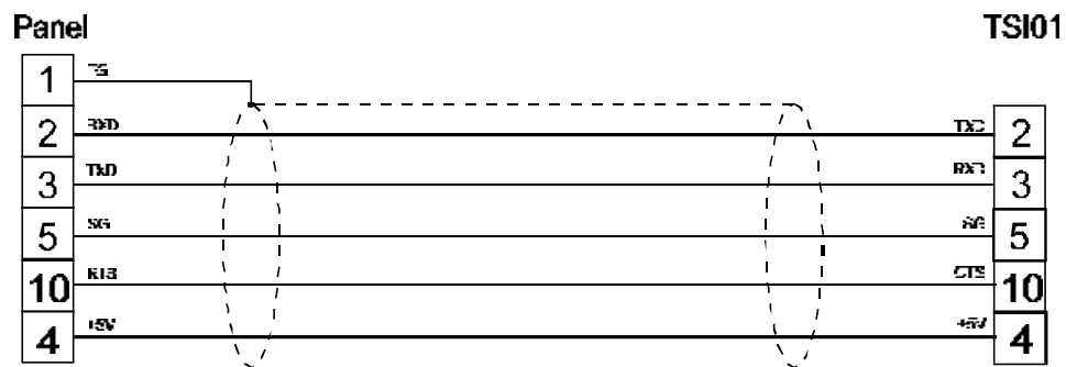
figure 1. Cable diagram
