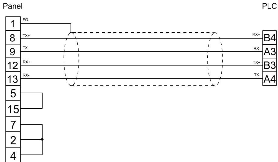
figure 1. Cable diagram
