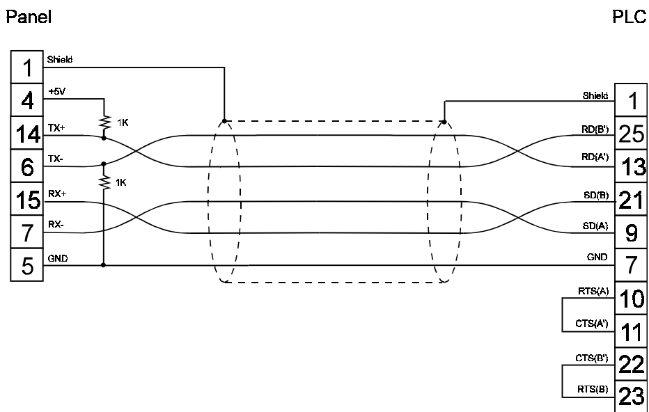
figure 1. Cable diagram
