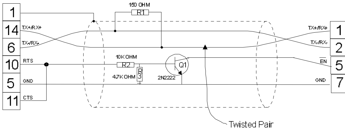
figure 1. Cable diagram
