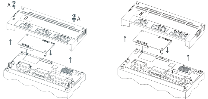
Figure 2 – Mounting AUX port module.
