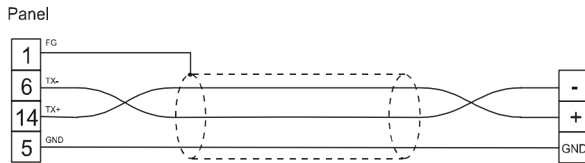
Figure 1. Cable diagram
