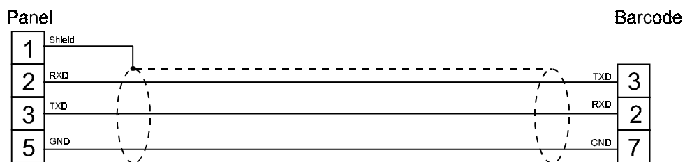
figure 1. Cable diagram
