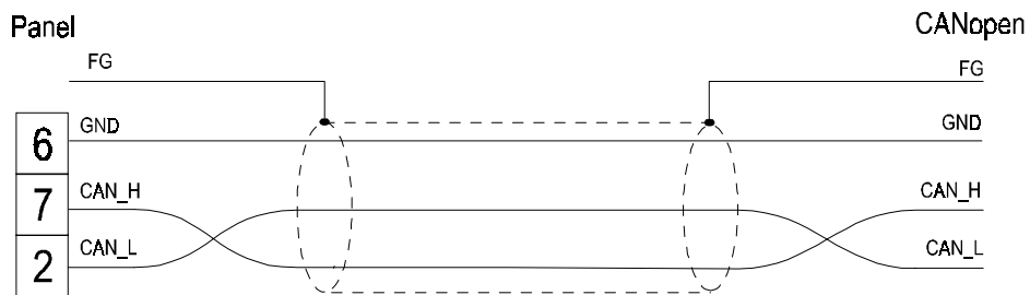
Figure 1. Cable diagram
