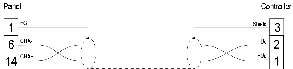
Figure 1. Cable diagram
