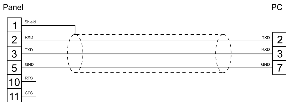
figure 1. Cable diagram
