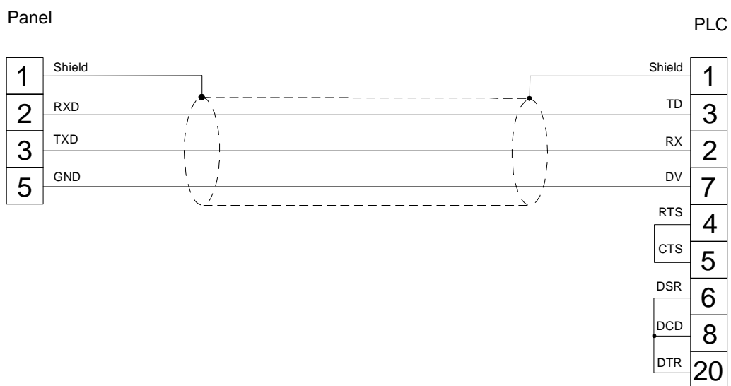
figure 1. Cable diagram
