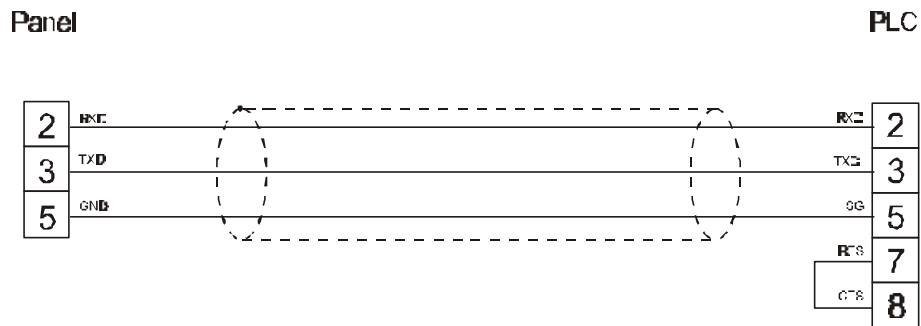
figure 1. Cable diagram
